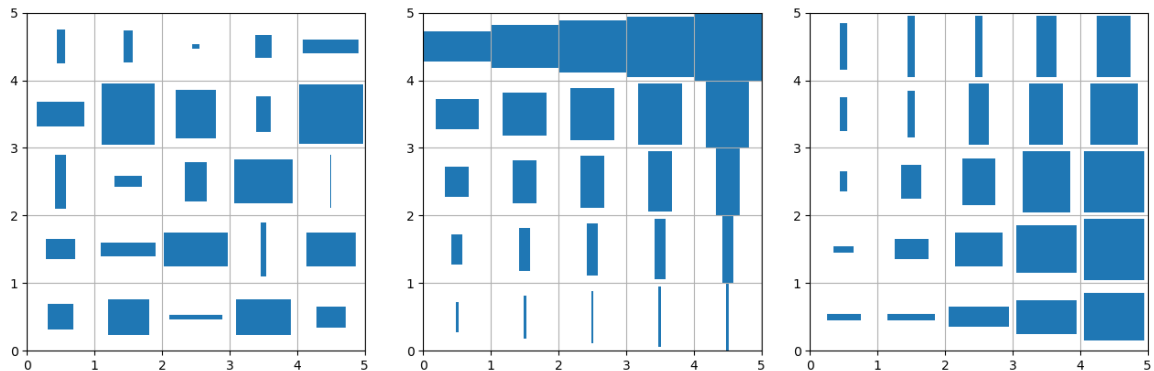
(a) Example of a dataset containing rectangles with width w and height h from the uniform distribution U(0, 1)
